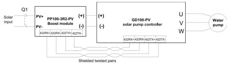
Connection between the boost module and solar pump controller
