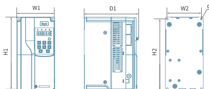
AC 3PH 380V 11~45kW mounting diagram
